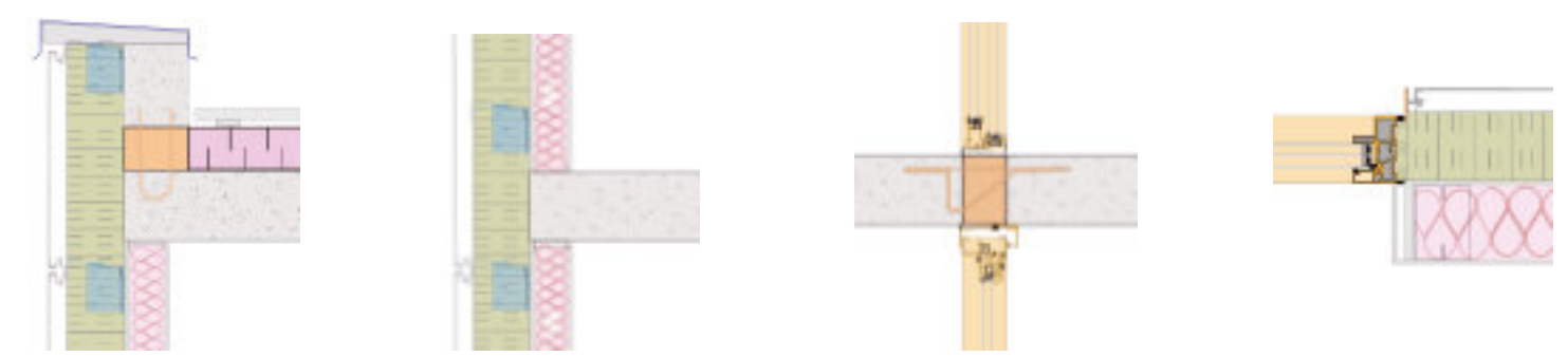
Roof to Wall Intermediate Floor Cantilevered Balcony Window to Wall
