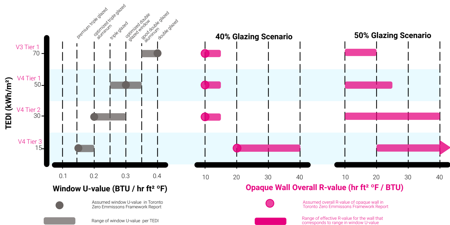
Figure 3. Optimization of the Vertical Facade A range of glazing and opaque performance will meet each tier or step for a multi-unit residential building with a complex shape for performance-based standards such as the Toronto Green Standard. 3,4
